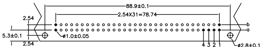
P.C. Board Layout
